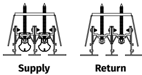
Supply
